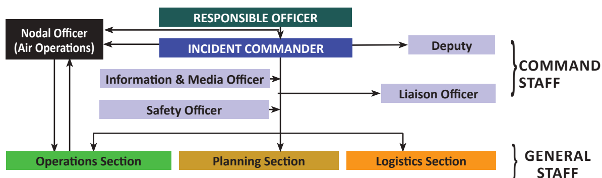
Fig. 1. IRS Organization
